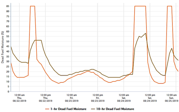
Forecast chart of 1-hour and 10-hour dead fuel moisture for Woodward from OK-FIRE.
