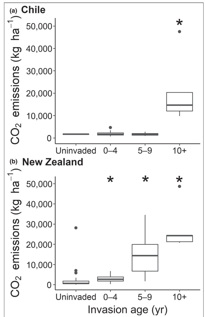
Figure 2. Simulated carbon dioxide emissions as a function of time since lodgepole pine ( Pinus contorta ) invasion (years) and in comparison to uninvaded plots in grassland systems, at sites in Chile (a) and New Zealand (b). Horizontal lines within boxes depict median values, boxes represent the interquartile range (25th–75th percentiles), whiskers (vertical lines) represent 1.5×interquartile range, and solid circles depict outliers. Asterisks highlight groups that were significantly higher ( P < 0.05 ) than the uninvaded plots based on post-hoc Tukey's tests.
